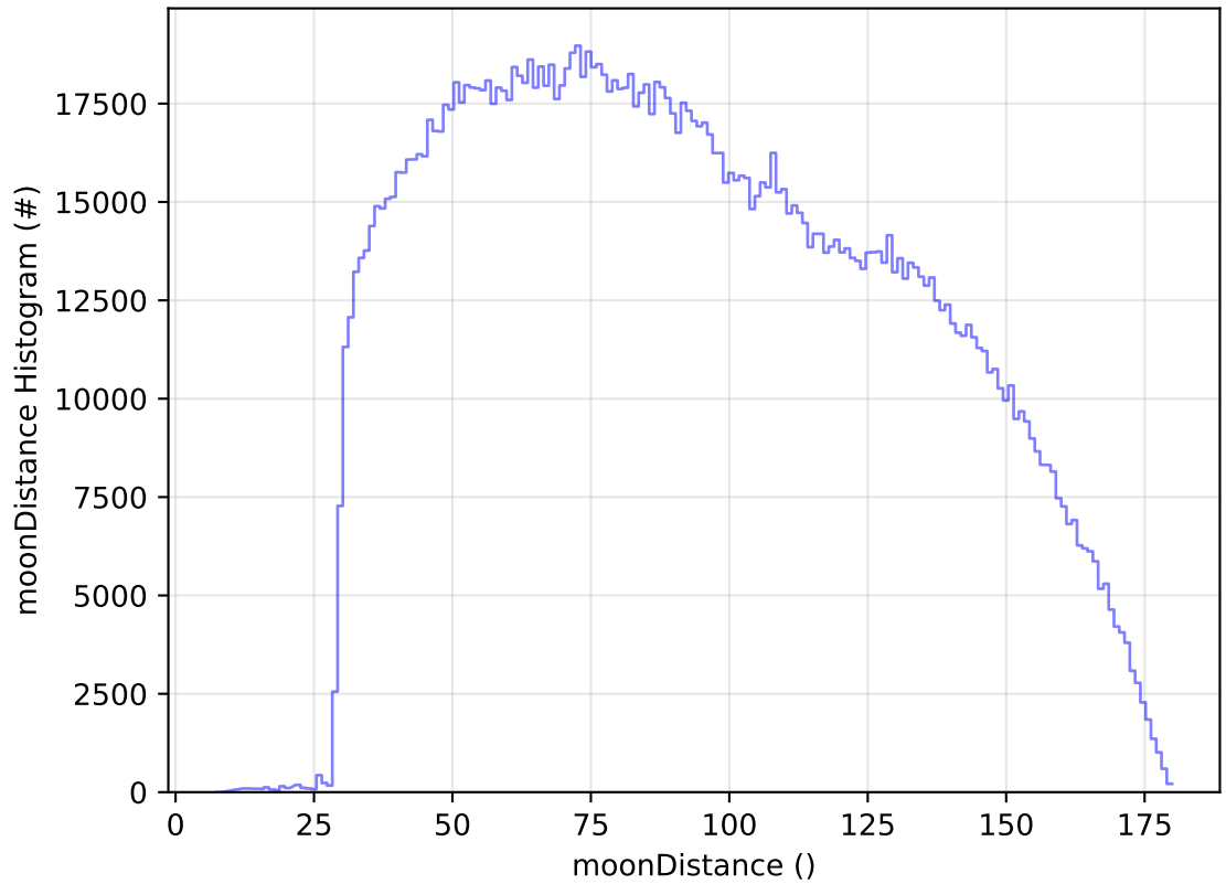
ddf_acor_sf10_lsf40_lsr50_v3.4_10yrs All sky all bands: moonDistance Histogram
