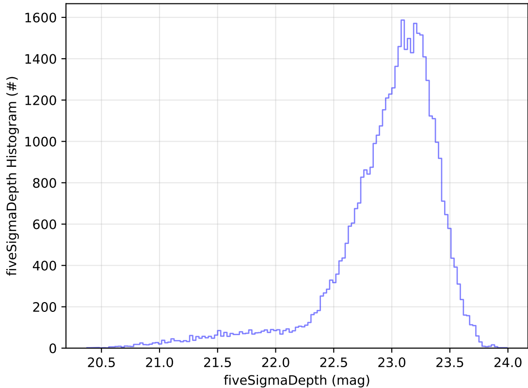
ddf_acor_sf10_lsf40_lsr50_v3.4_10yrs Yr 1 z band: fiveSigmaDepth Histogram
