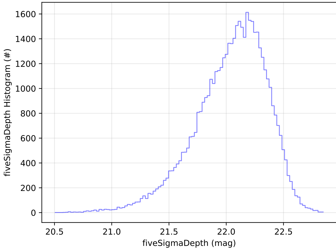
ddf_acor_sf10_lsf40_lsr50_v3.4_10yrs Yr 1 y band: fiveSigmaDepth Histogram
