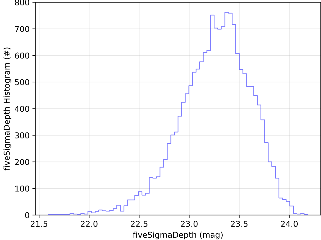
ddf_acor_sf10_lsf40_lsr50_v3.4_10yrs Yr 1 u band: fiveSigmaDepth Histogram
