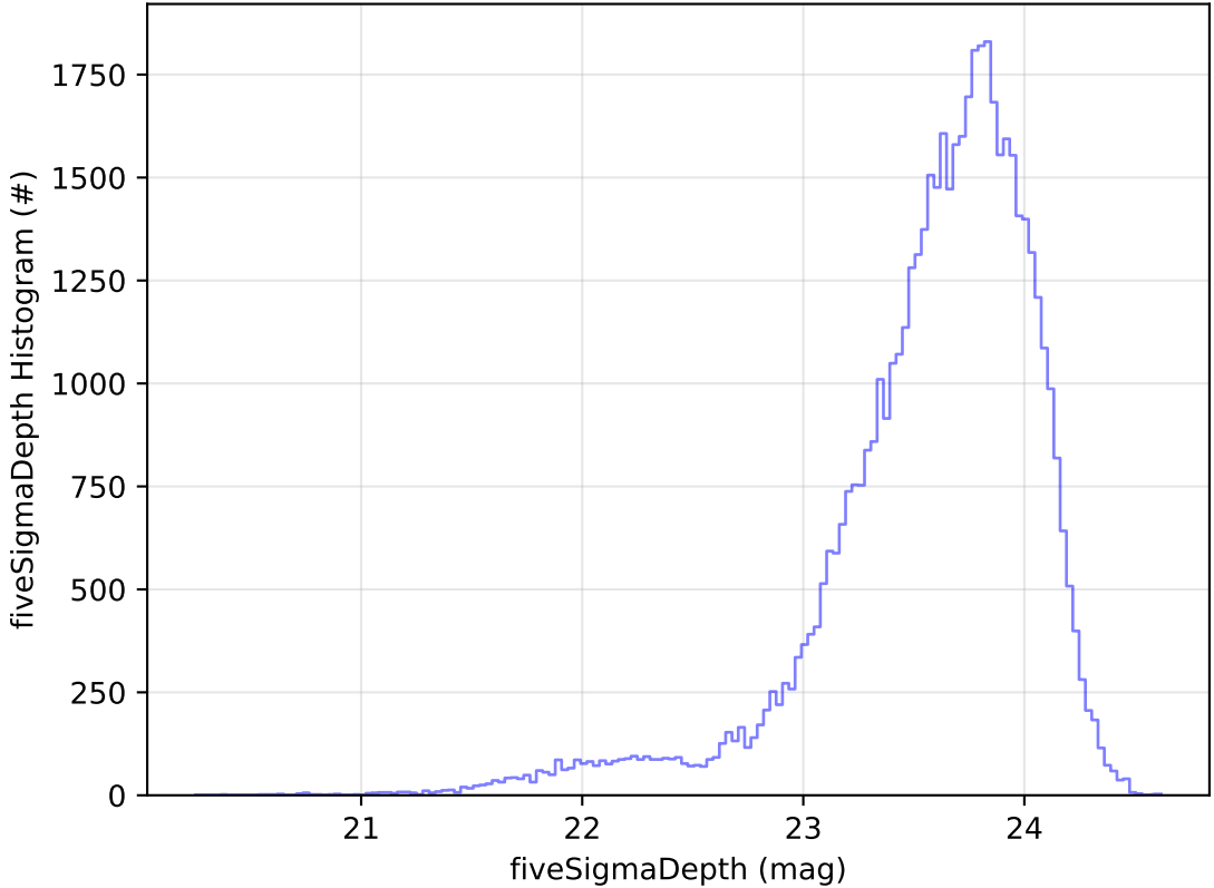
ddf_acor_sf10_lsf40_lsr50_v3.4_10yrs Yr 1 i band: fiveSigmaDepth Histogram
