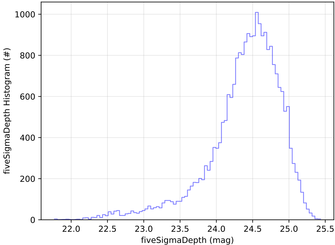
ddf_acor_sf10_lsf40_lsr50_v3.4_10yrs Yr 1 g band: fiveSigmaDepth Histogram
