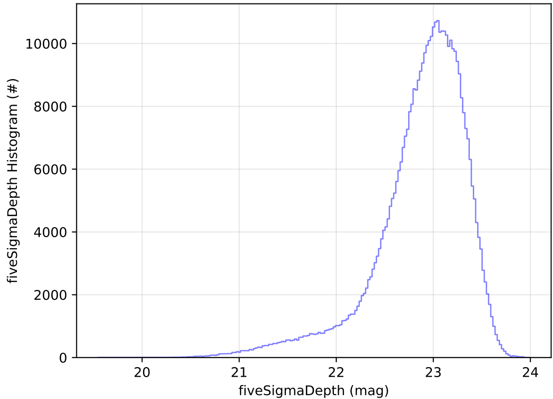
ddf_acor_sf10_lsf40_lsr50_v3.4_10yrs WFD z band: fiveSigmaDepth Histogram
