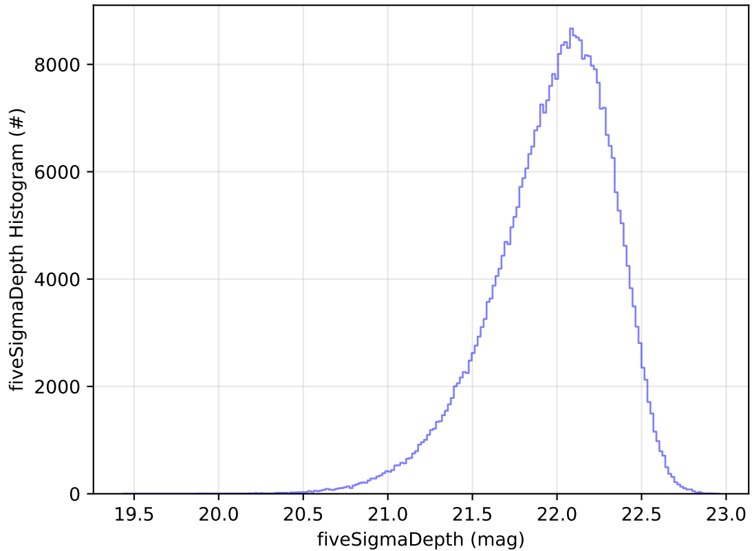
ddf_acor_sf10_lsf40_lsr50_v3.4_10yrs WFD y band: fiveSigmaDepth Histogram
