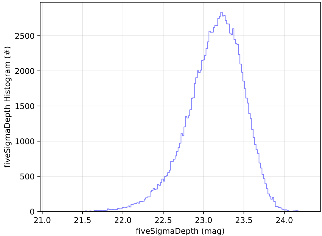
ddf_acor_sf10_lsf40_lsr50_v3.4_10yrs WFD u band: fiveSigmaDepth Histogram
