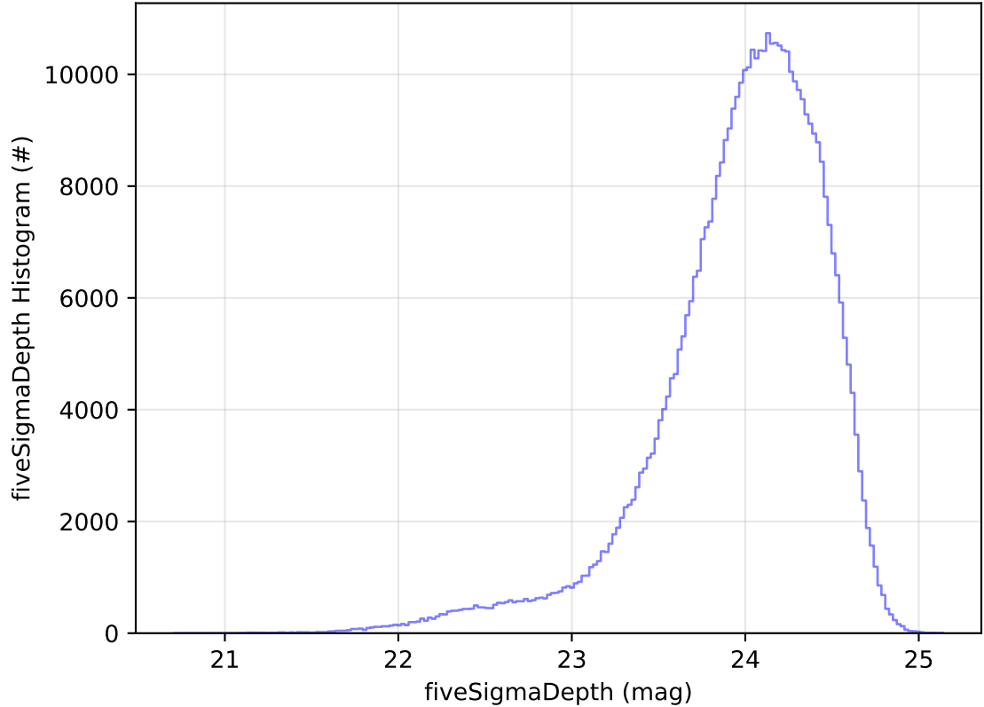
ddf_acor_sf10_lsf40_lsr50_v3.4_10yrs WFD r band: fiveSigmaDepth Histogram
