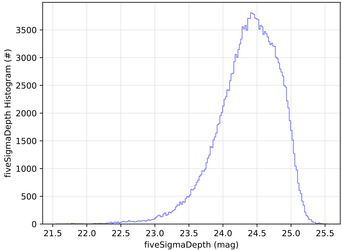
ddf_acor_sf10_lsf40_lsr50_v3.4_10yrs WFD g band: fiveSigmaDepth Histogram
