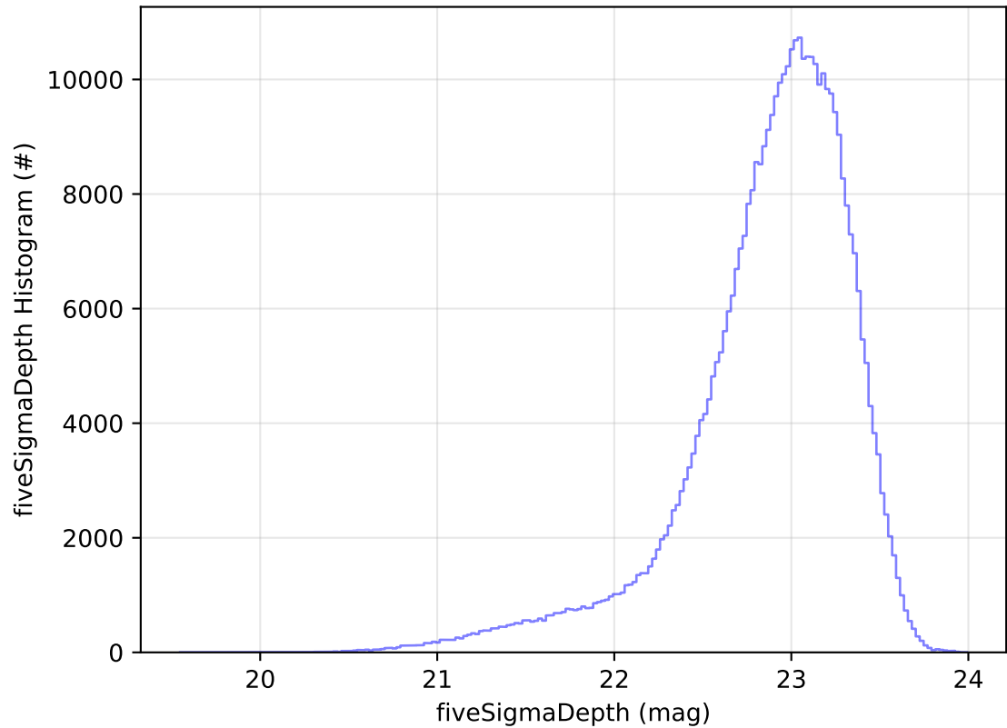
ddf_acor_sf10_lsf40_lsr50_v3.4_10yrs All sky z band: fiveSigmaDepth Histogram
