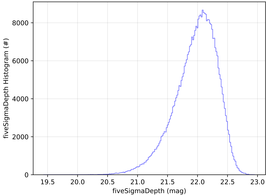
ddf_acor_sf10_lsf40_lsr50_v3.4_10yrs All sky y band: fiveSigmaDepth Histogram
