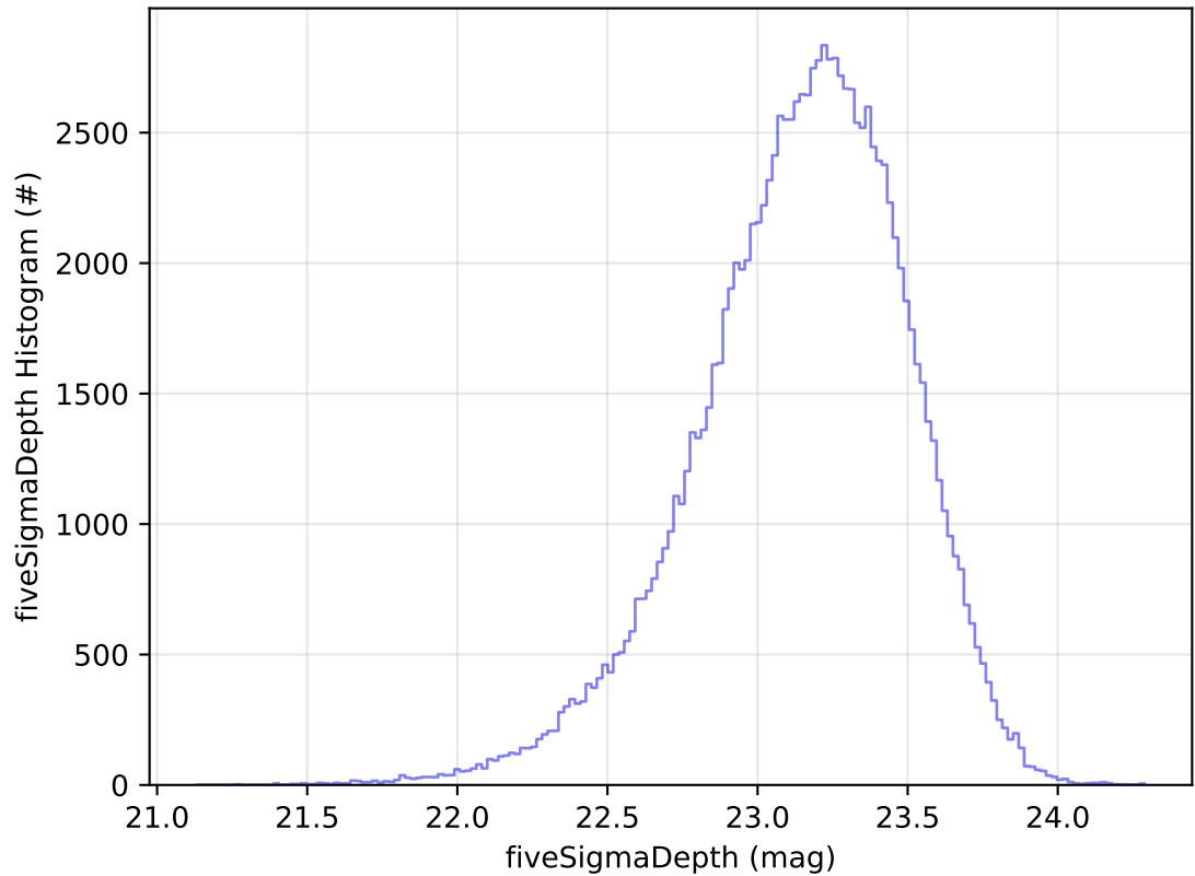
ddf_acor_sf10_lsf40_lsr50_v3.4_10yrs All sky u band: fiveSigmaDepth Histogram
