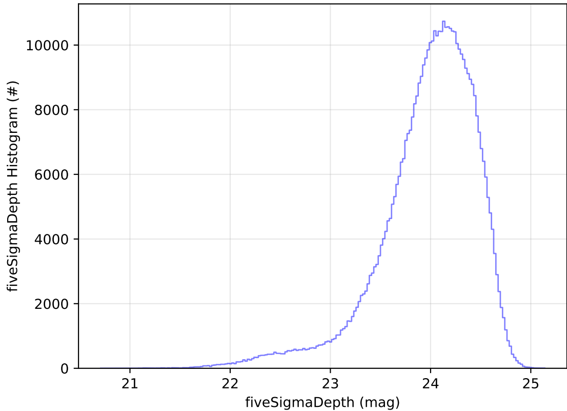
ddf_acor_sf10_lsf40_lsr50_v3.4_10yrs All sky r band: fiveSigmaDepth Histogram
