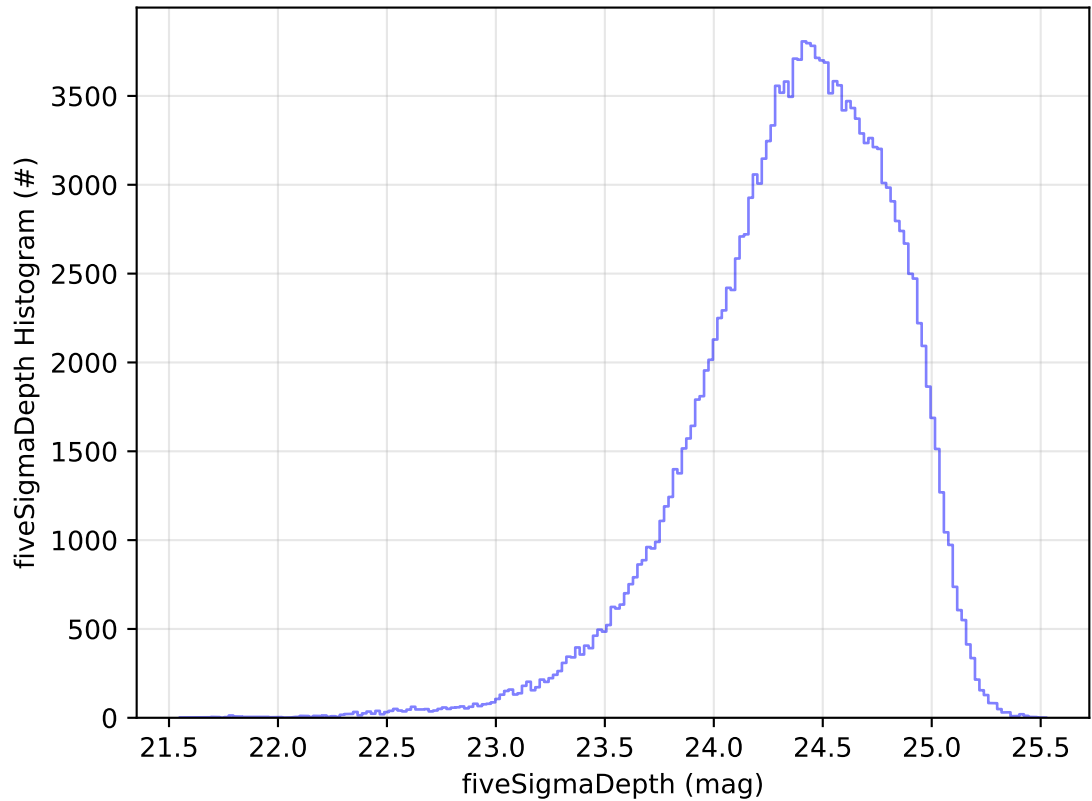
ddf_acor_sf10_lsf40_lsr50_v3.4_10yrs All sky g band: fiveSigmaDepth Histogram
