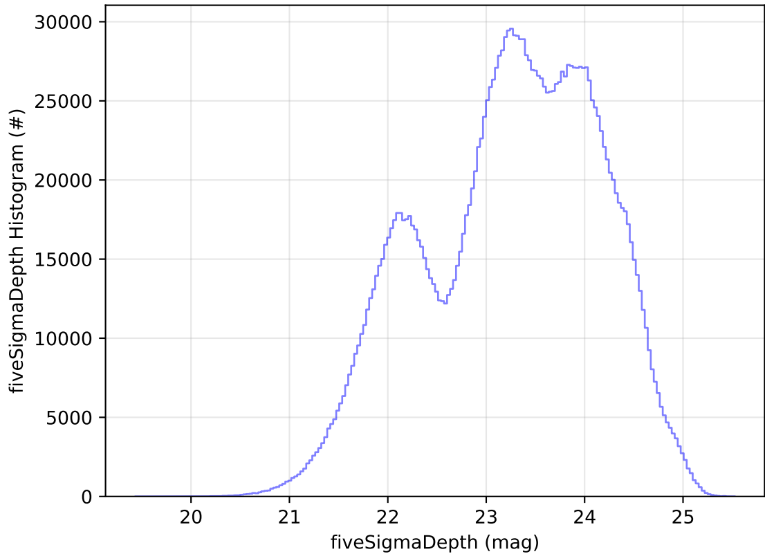
ddf_acor_sf10_lsf40_lsr50_v3.4_10yrs All sky all bands: fiveSigmaDepth Histogram
