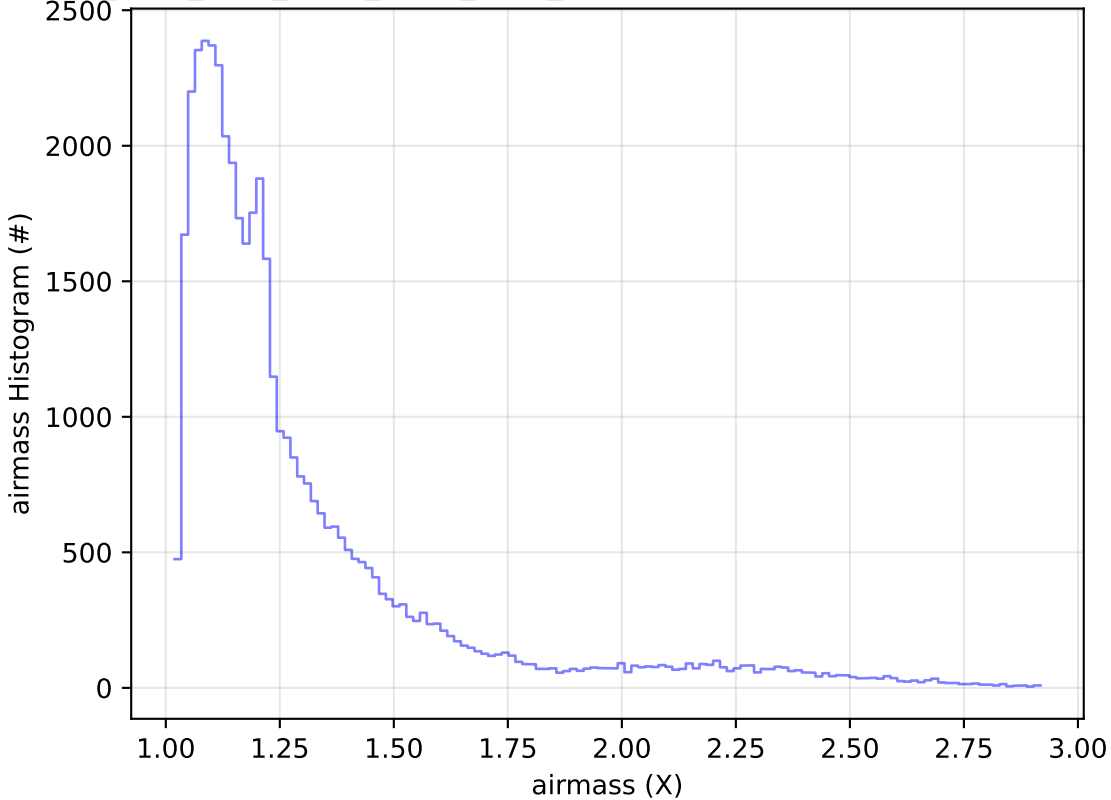
ddf_acor_sf10_lsf40_lsr50_v3.4_10yrs Yr 1 z band: airmass Histogram
