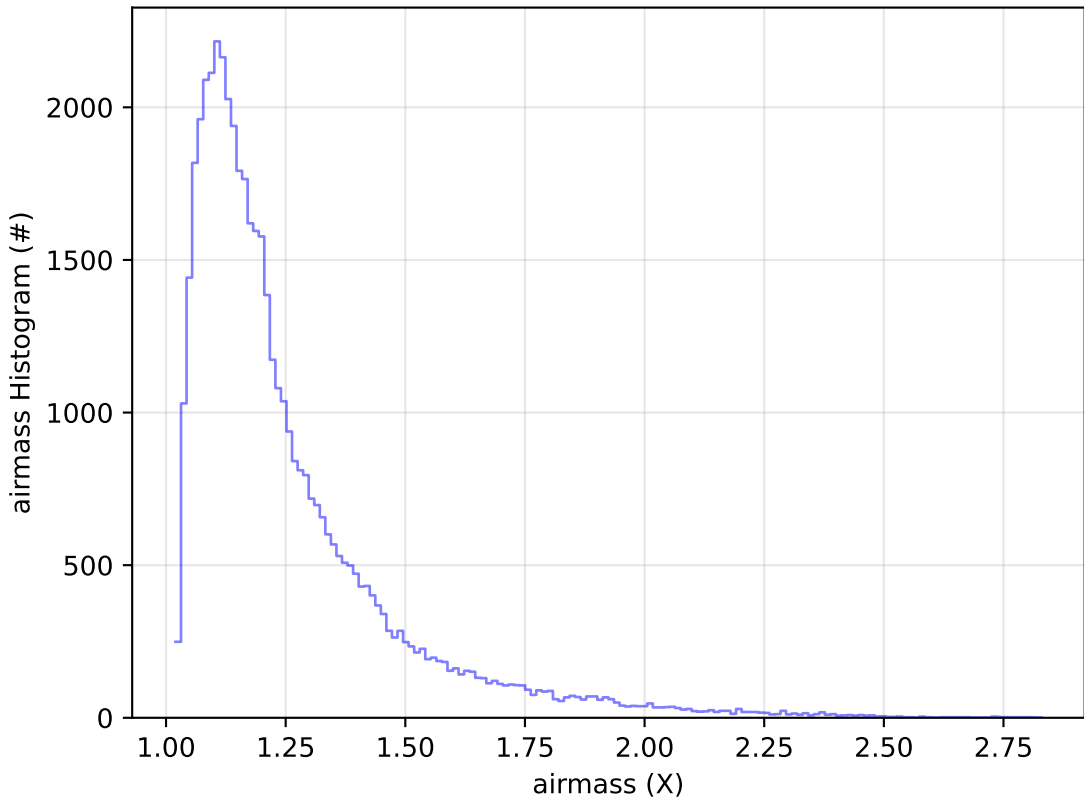
ddf_acor_sf10_ls40_lsr50_v3.4_10yrs Yr 1 y band: airmass Histogram
