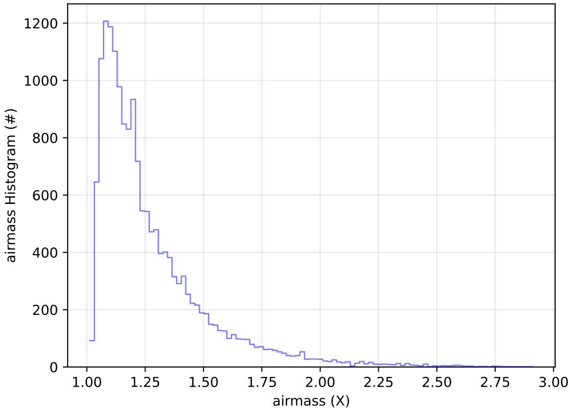
ddf_acor_sf10_lsf40_lsr50_v3.4_10yrs Yr 1 u band: airmass Histogram
