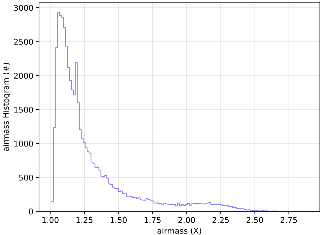
ddf_acor_sf10_lsf40_lsr50_v3.4_10yrs Yr 1 r band: airmass Histogram
