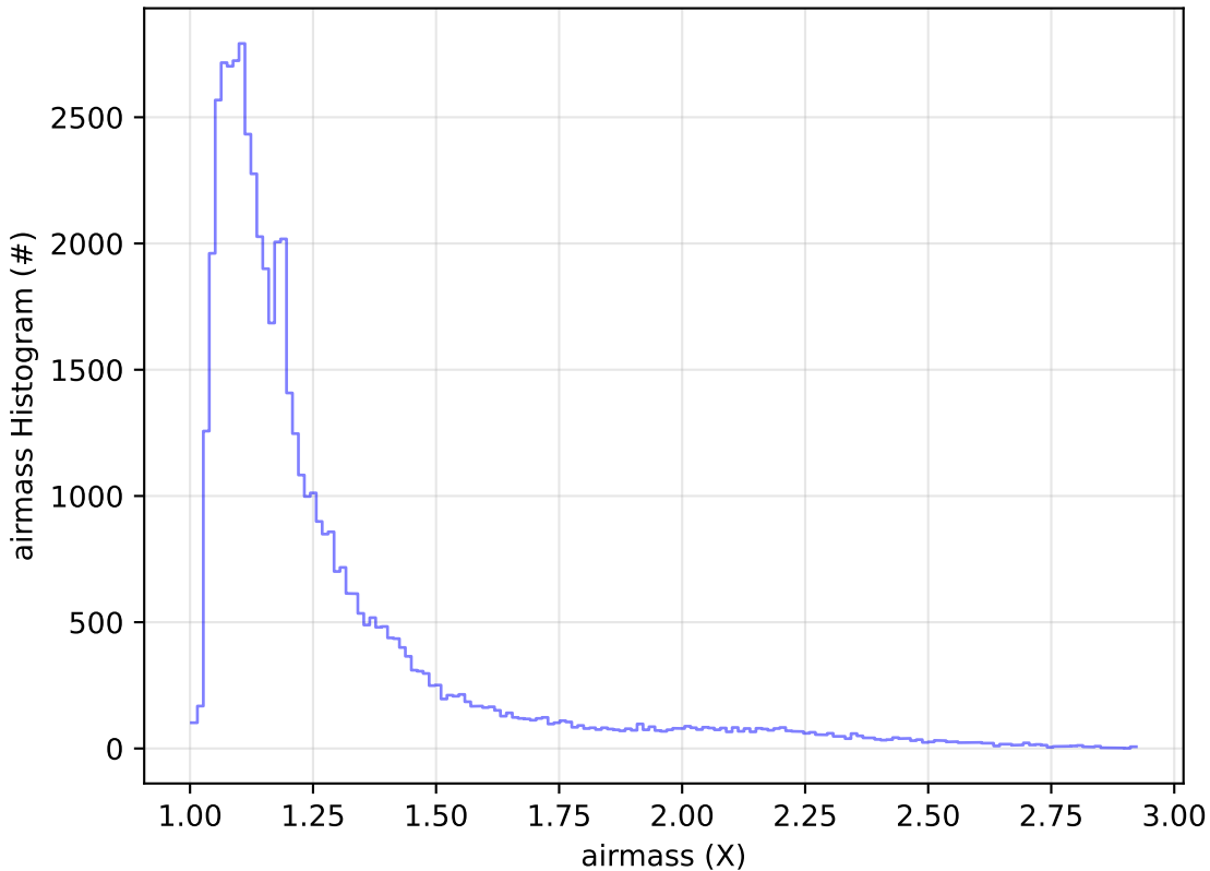
ddf_acor_sf10_lsf40_lsr50_v3.4_10yrs Yr 1 i band: airmass Histogram
