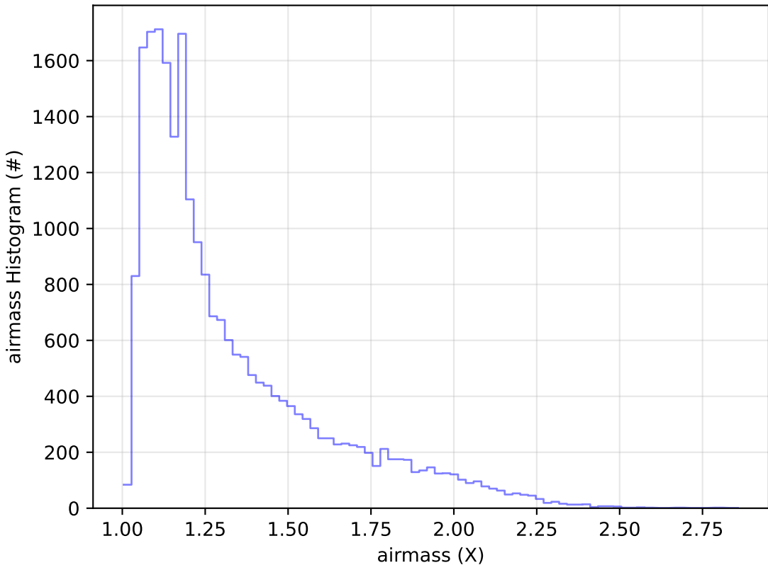
ddf_acor_sf10_lsf40_lsr50_v3.4_10yrs Yr 1 g band: airmass Histogram
