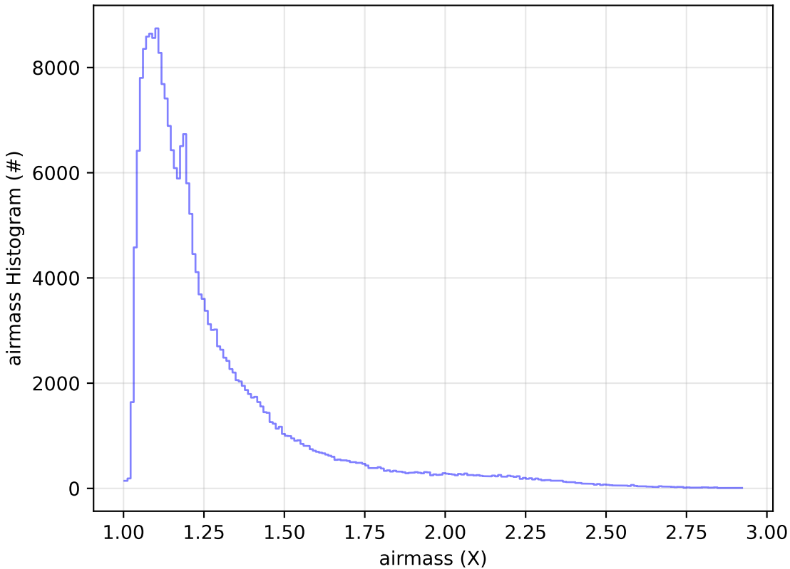
ddf_acor_sf10_lsf40_lsr50_v3.4_10yrs Yr 1 all bands: airmass Histogram
