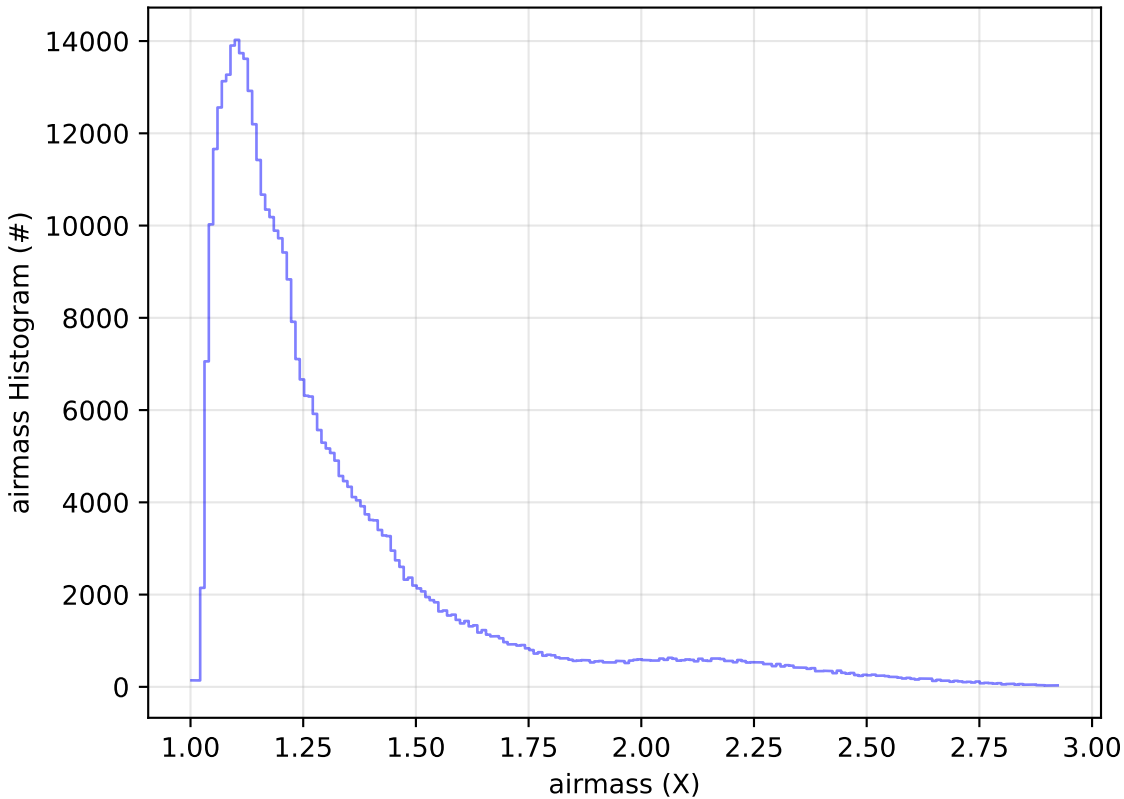
ddf_acor_sf10_lsf40_lsr50_v3.4_10yrs WFD z band: airmass Histogram
