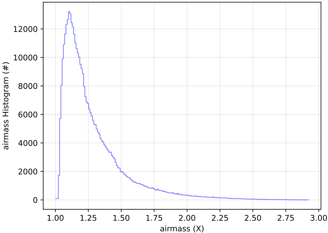
ddf_acor_sf10_lsf40_lsr50_v3.4_10yrs WFD y band: airmass Histogram
