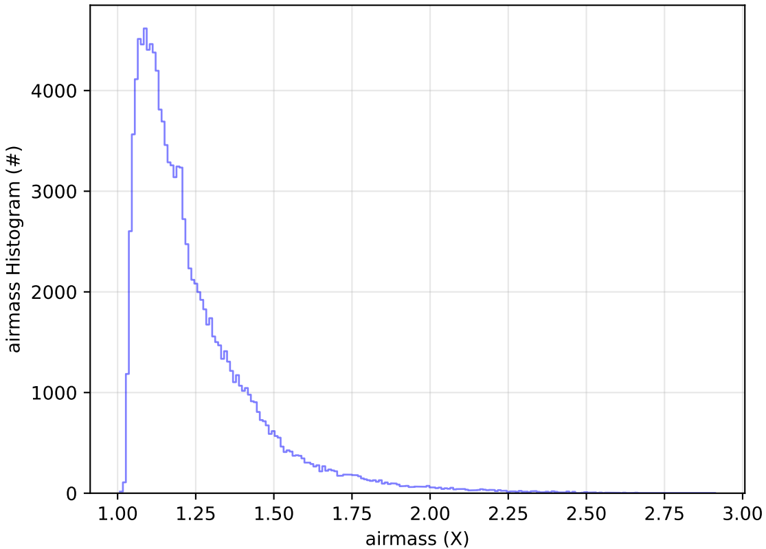
ddf_acor_sf10_lsf40_lsr50_v3.4_10yrs WFD u band: airmass Histogram
