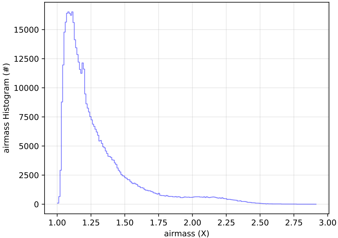
ddf_acor_sf10_Isf40_Isr50_v3.4_10yrs WFD r band: airmass Histogram
