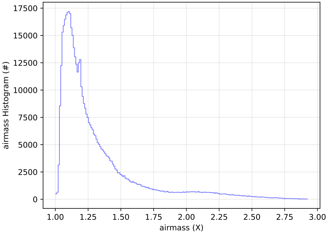
ddf_acor_sf10_lsf40_lsr50_v3.4_10yrs WFD i band: airmass Histogram
