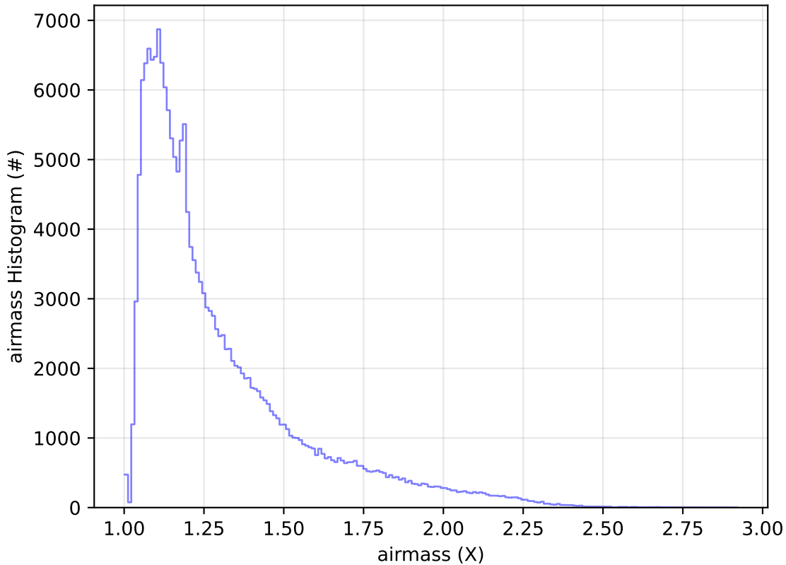
ddf_acor_sf10_lsf40_lsr50_v3.4_10yrs WFD g band: airmass Histogram
