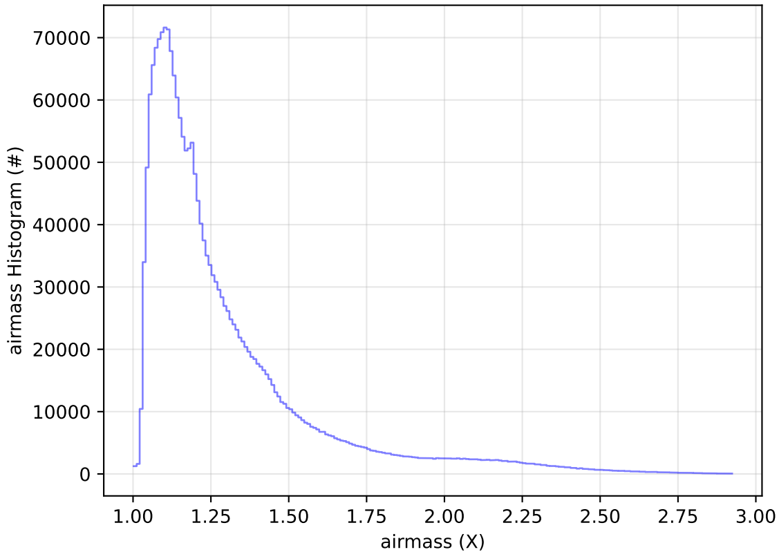
ddf_acor_sf10_lsf40_lsr50_v3.4_10yrs WFD all bands: airmass Histogram
