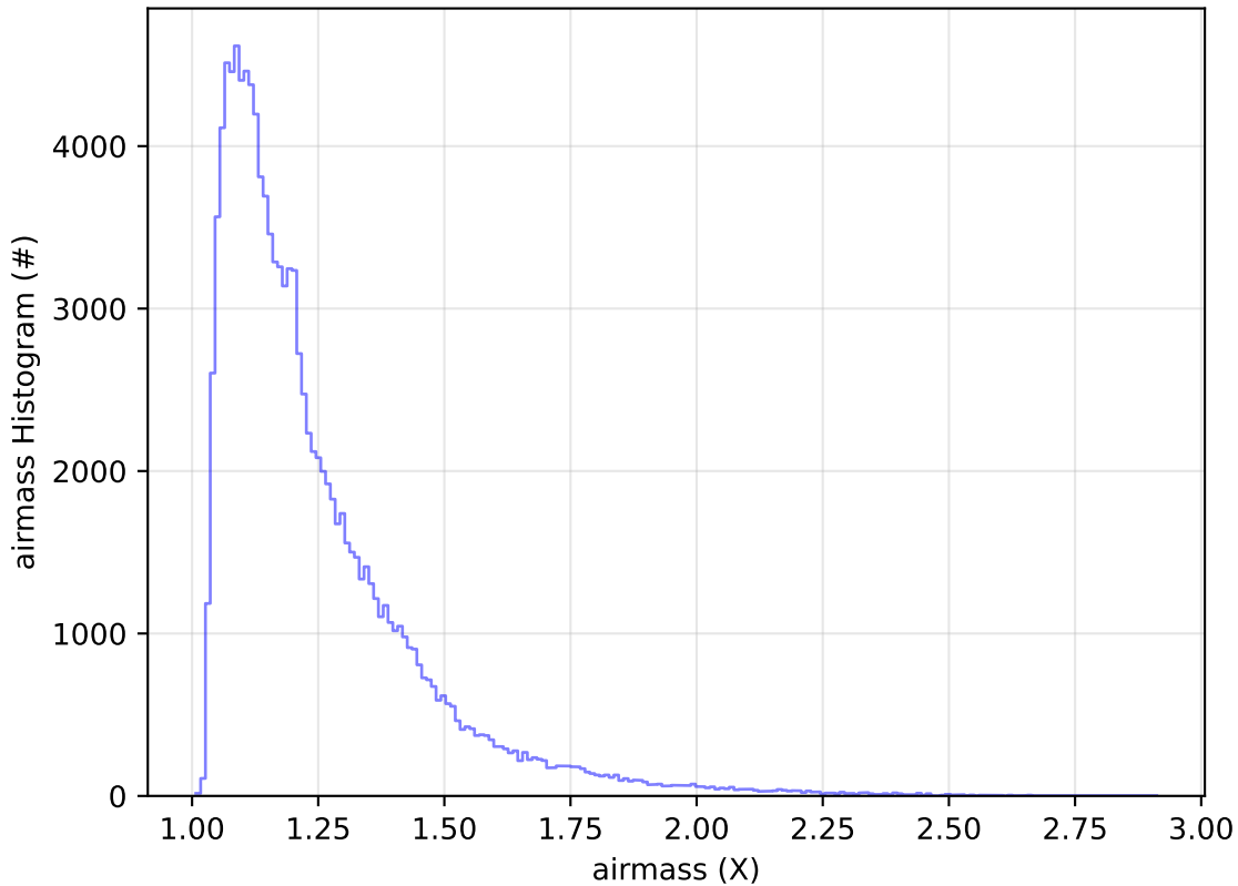
ddf_acor_sf10_lsf40_lsr50_v3.4_10yrs All sky u band: airmass Histogram
