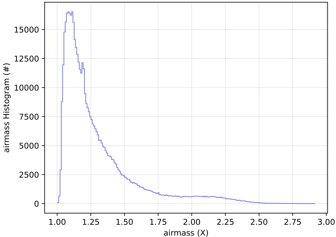
ddf_acor_sf10_lsf40_lsr50_v3.4_10yrs All sky r band: airmass Histogram
