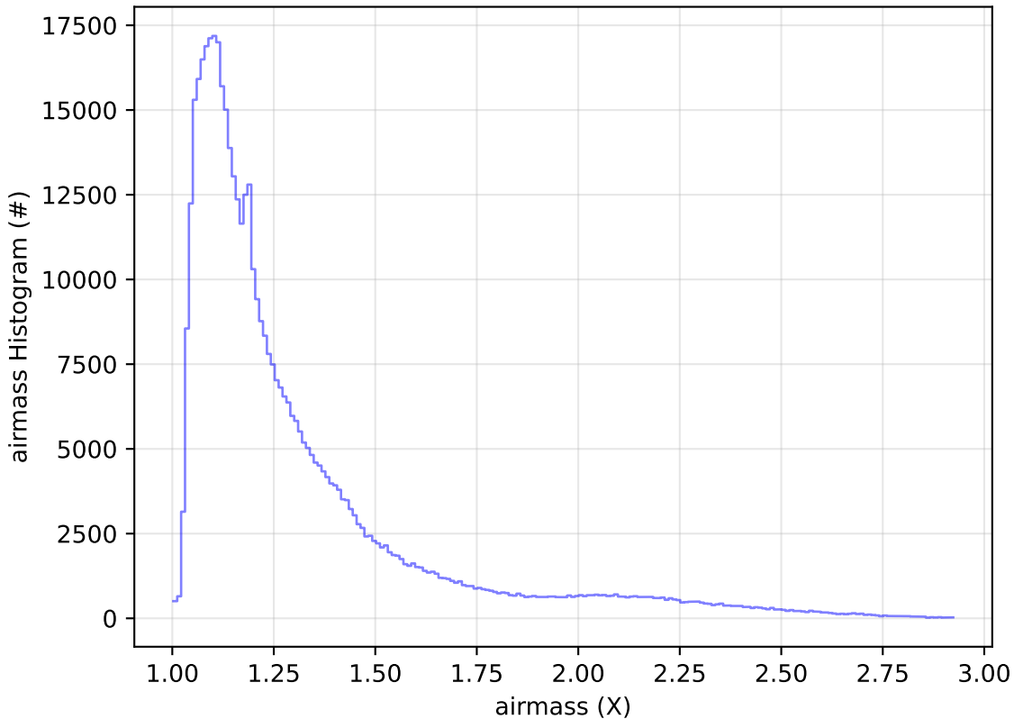
ddf_acor_sf10_lsf40_lsr50_v3.4_10yrs All sky i band: airmass Histogram
