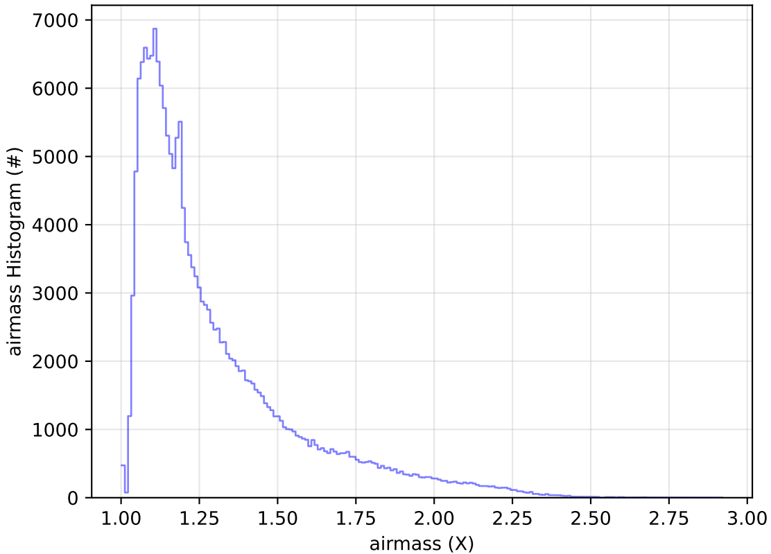
ddf_acor_sf10_lsf40_lsr50_v3.4_10yrs All sky g band: airmass Histogram
