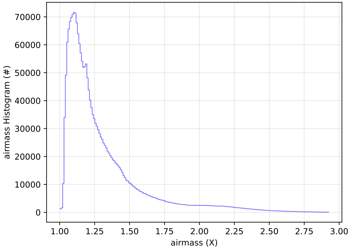
ddf_acor_sf10_lsf40_lsr50_v3.4_10yrs All sky all bands: airmass Histogram
