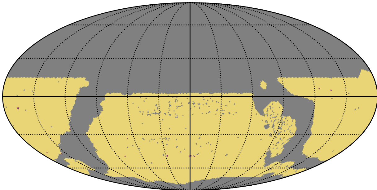
ddf_acor_sf10_lsf40_lsr50_v3.4_10yrs WFD: RapidRevisits
