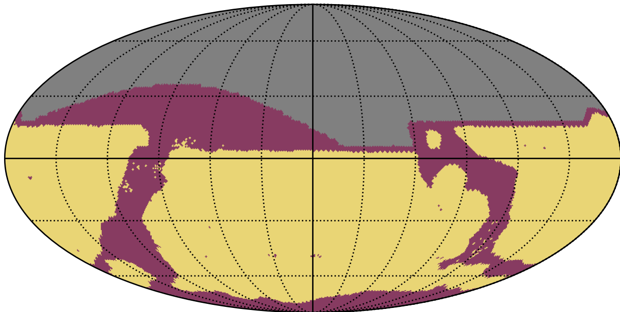
ddf_acor_sf10_lsf40_lsr50_v3.4_10yrs All sky: RapidRevisits
