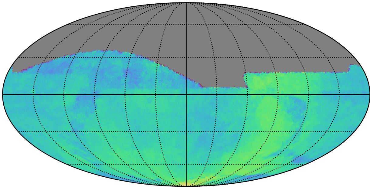
ddf_acor_sf10_lsf40_lsr50_v3.4_10yrs All sky: Parallax Coverage @ 22.4
