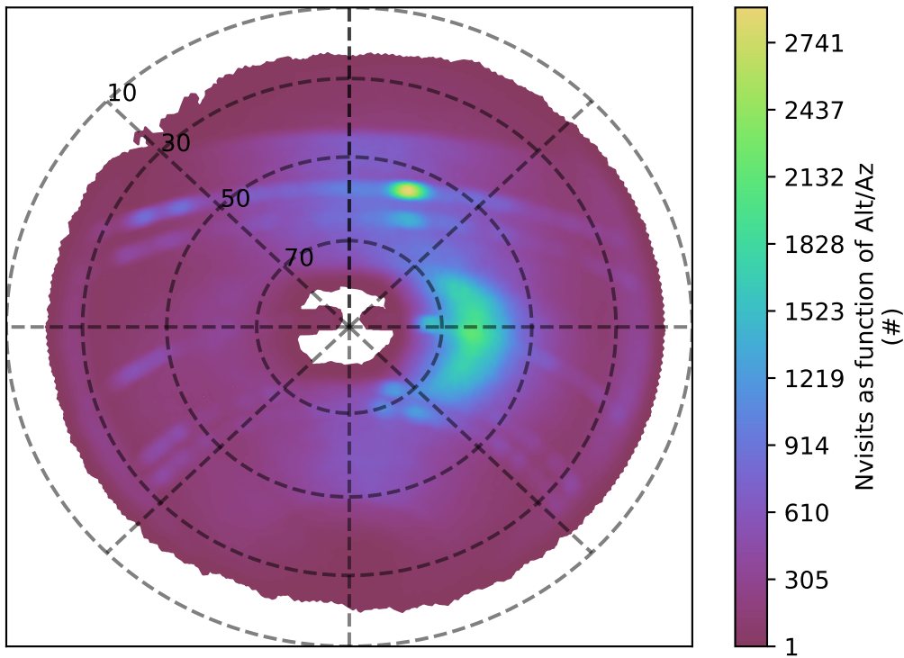
ddf_acor_sf10_lsf40_lsr50_v3.4_10yrs z band: Nvisits as function of Alt/Az
