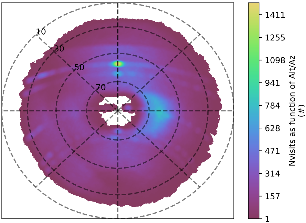
ddf_acor_sf10_lsf40_lsr50_v3.4_10yrs g band: Nvisits as function of Alt/Az
