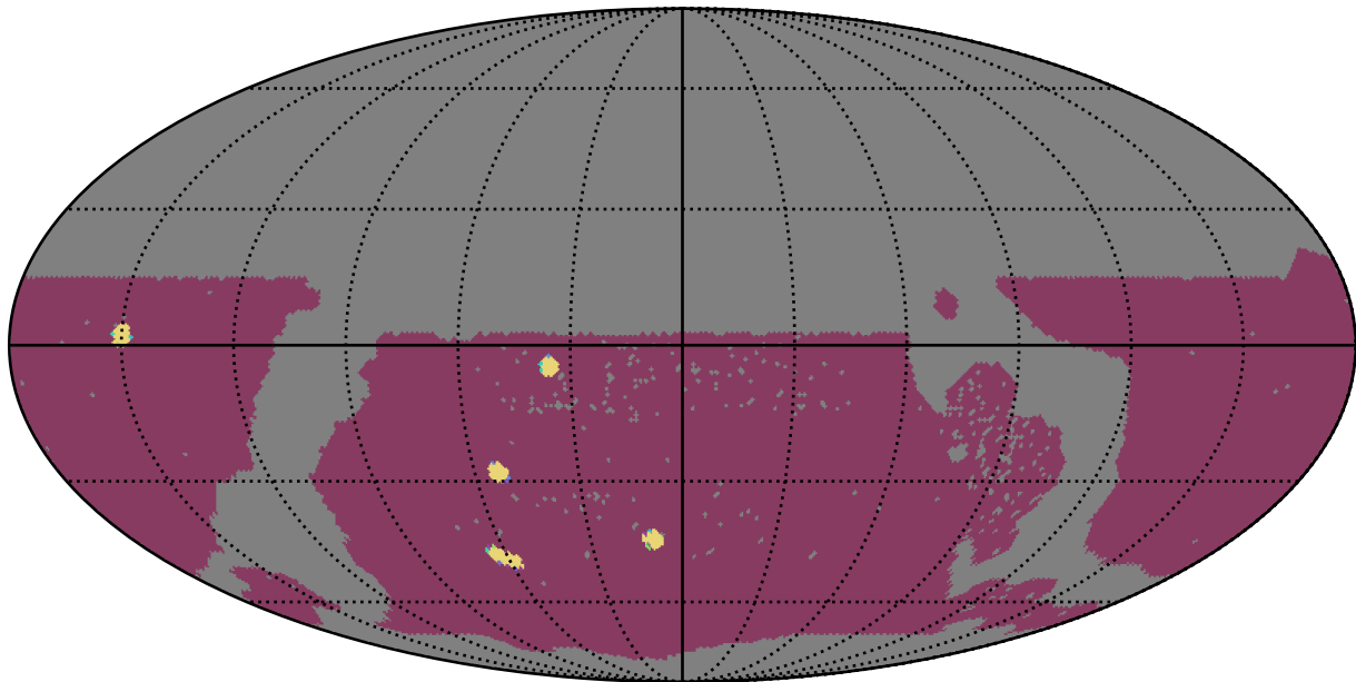
ddf_acor_sf10_lsf40_lsr50_v3.4_10yrs WFD: NumberOfQuickRevisits
