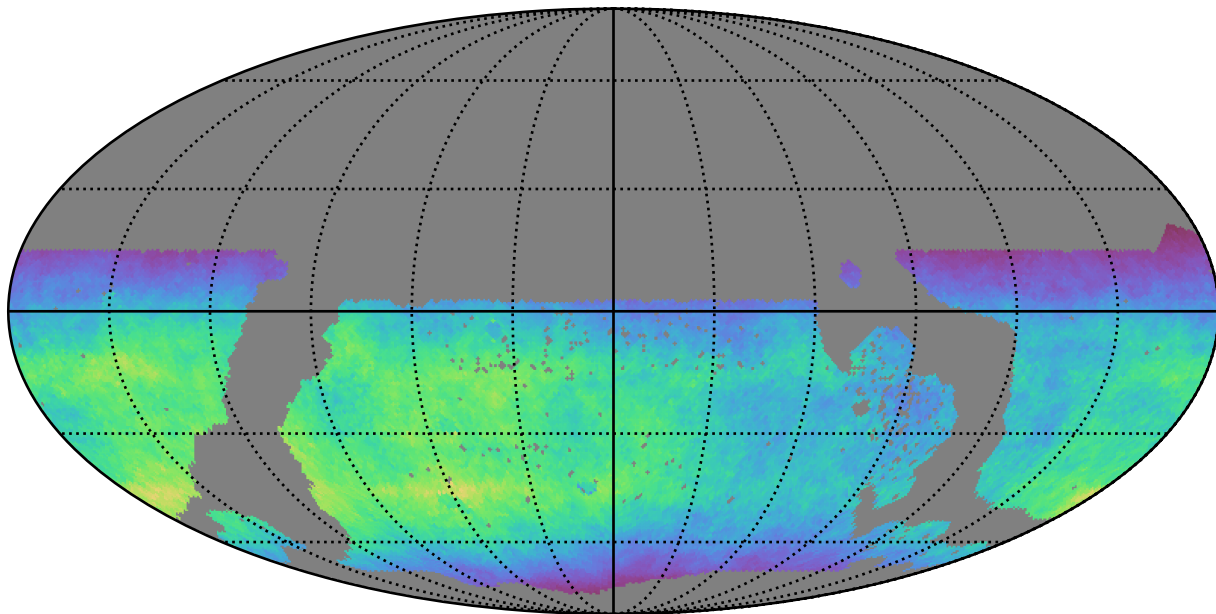
ddf_acor_sf10_lsf40_lsr50_v3.4_10yrs WFD y band: Normalized Teff
