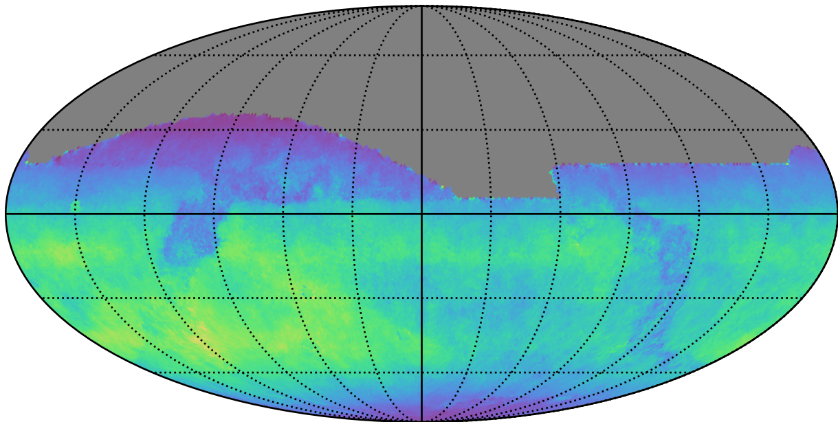
ddf_acor_sf10_lsf40_lsr50_v3.4_10yrs All sky z band: Normalized Teff
