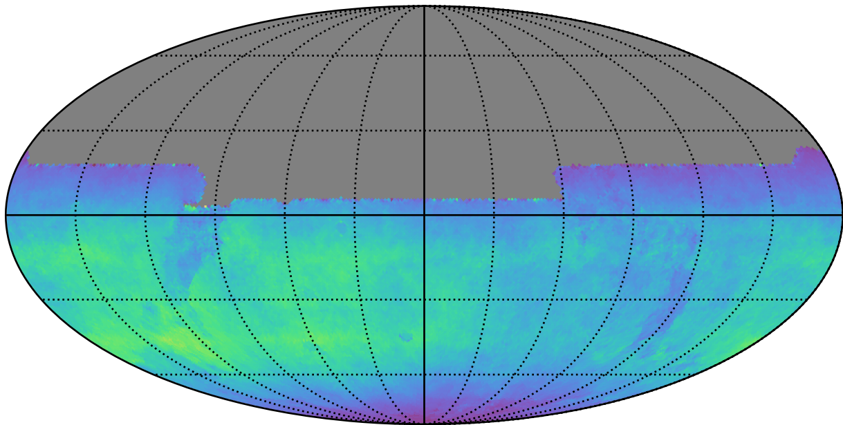
ddf_acor_sf10_lsf40_lsr50_v3.4_10yrs All sky y band: Normalized Teff
