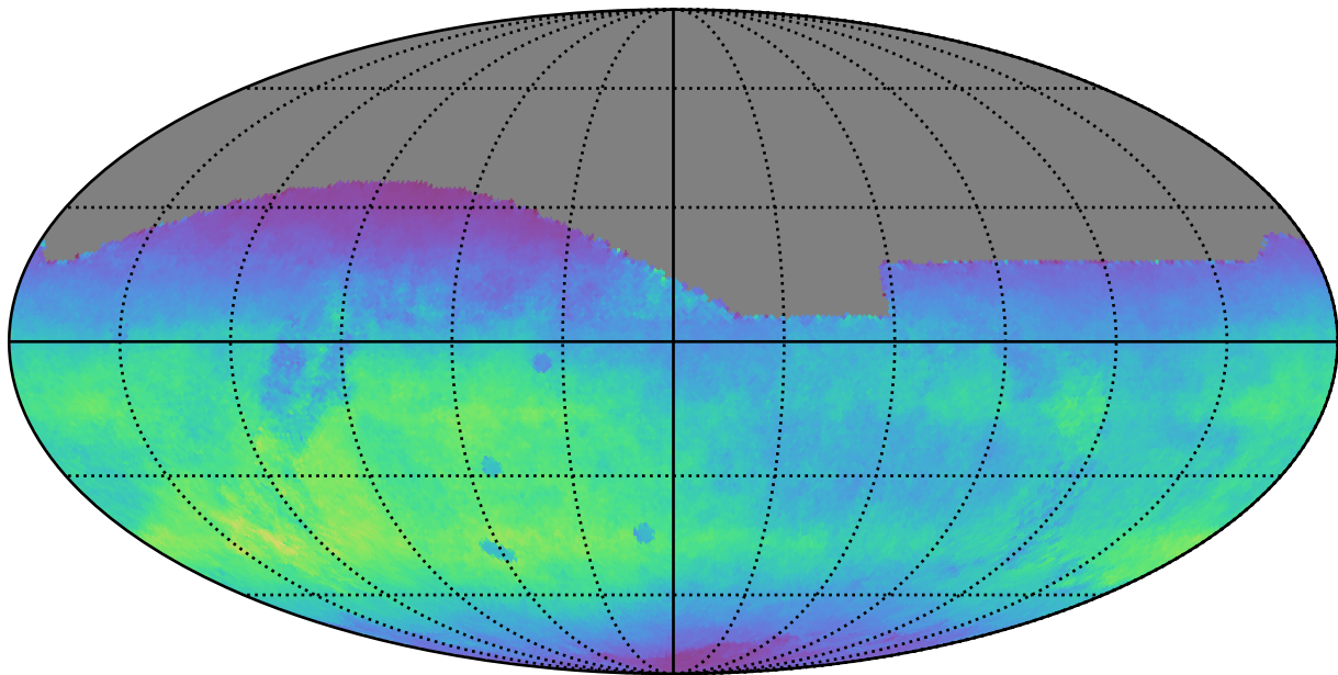
ddf_acor_sf10_lsf40_lsr50_v3.4_10yrs All sky r band: Normalized Teff
