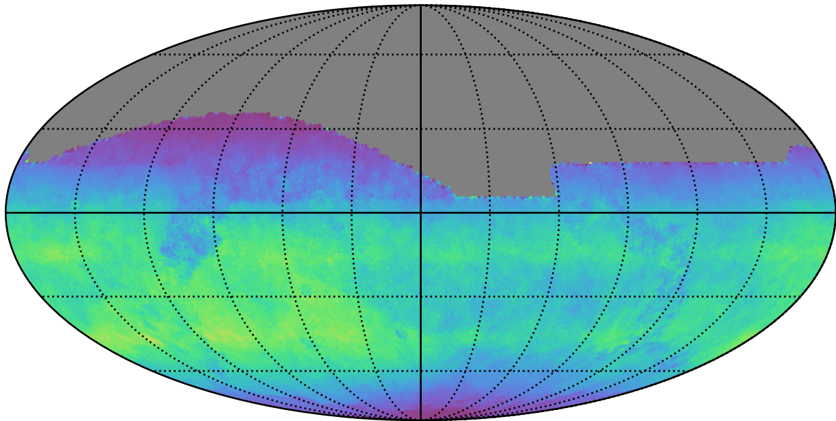
ddf_acor_sf10_lsf40_lsr50_v3.4_10yrs All sky i band: Normalized Teff
