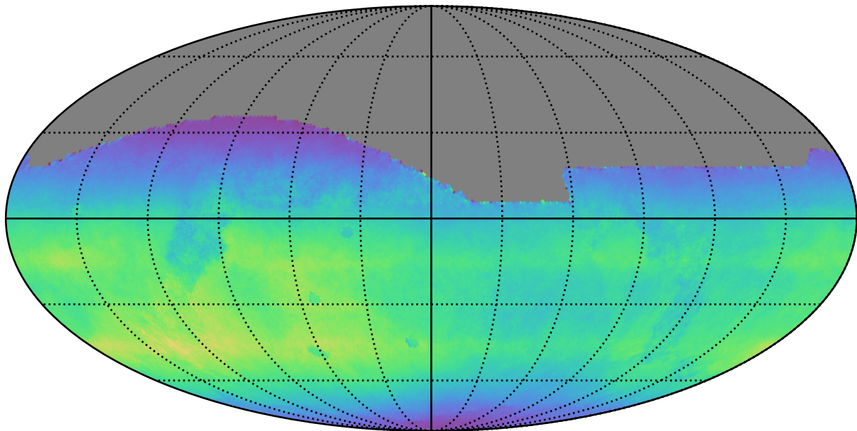
ddf_acor_sf10_lsf40_lsr50_v3.4_10yrs All sky all bands: Normalized Teff
