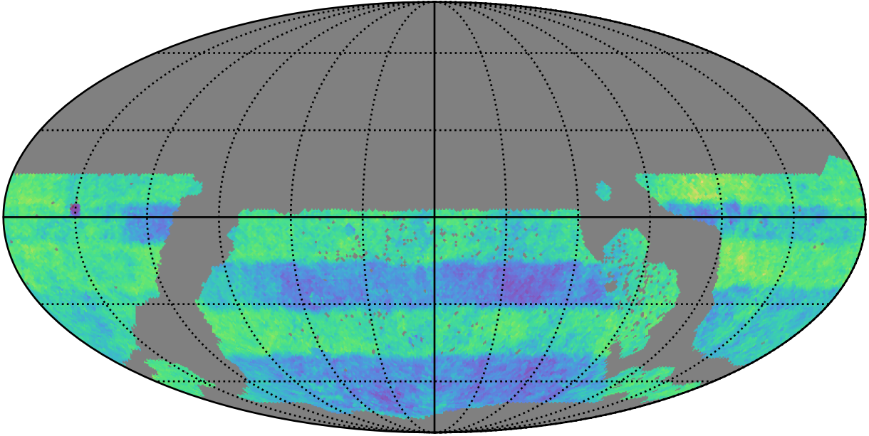
ddf_acor_sf10_lsf40_lsr50_v3.4_10yrs WFD: Normalized Proper Motion Uncert @ 24.0
