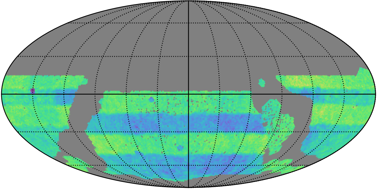
ddf_acor_sf10_lsf40_lsr50_v3.4_10yrs WFD: Normalized Proper Motion Uncert @ 20.5
